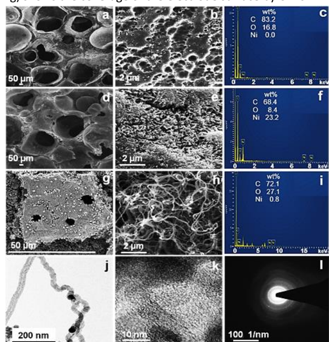
Fig. 1. SEM and EDX micrographs of (a-c) CF, (d-f) NiO-CF, and (g-i) NiO-CNF-CF. TEM images of NiO-CNF-CF at (j) low and (k) high resolutions, and (l) the corresponding SAED pattern.
